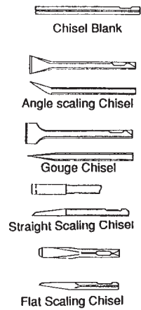
Figure 21.61 Common attachments for air scalars.
