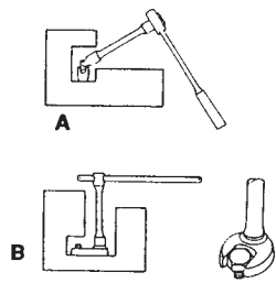
Figure 21.22 Useful socket items: A) Universal socket B) crowfoot attachment
