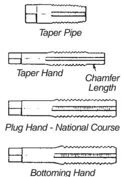
Figure 21.15 Types of common taps.
