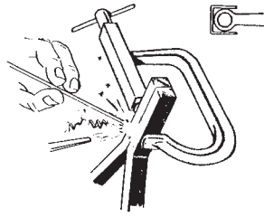
Figure 21.26 Welding C-clamp
