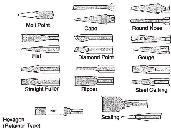
Figure 21.57 Chisel types
