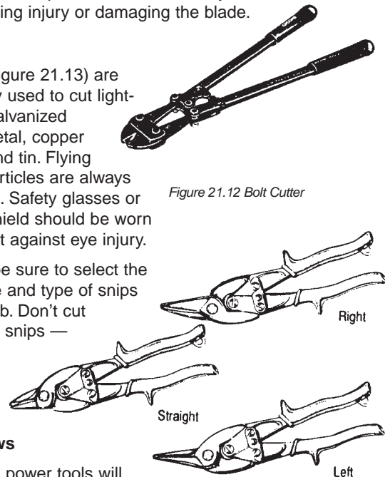
Figure 21.13 Snips
